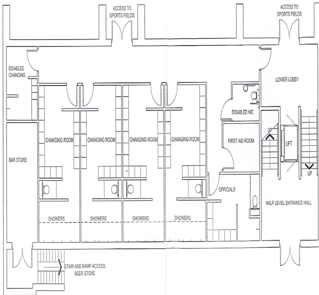
LOWER FLOOR PLAN : SCALE 1/100
